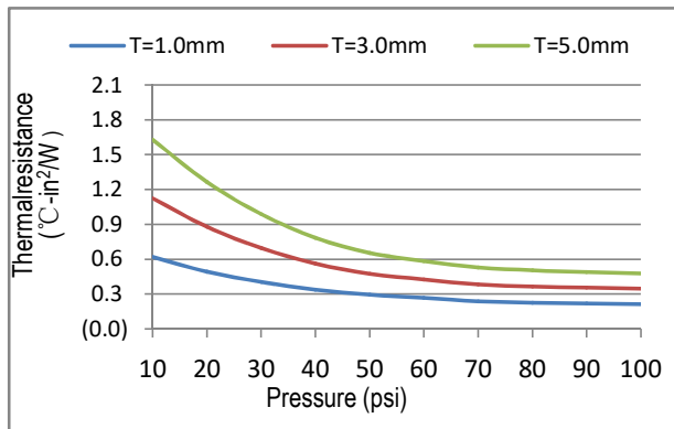
Pressure. vs. Thermal Resistance
